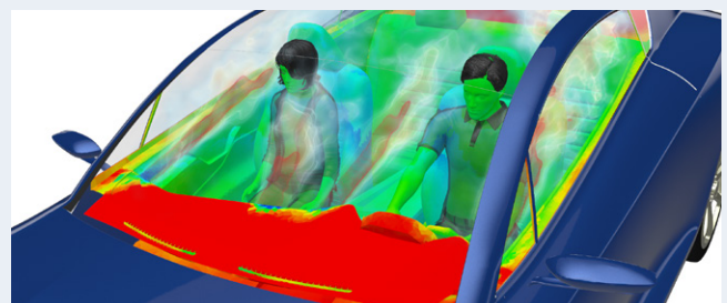
Long transient cabin PowerFLOW simulation for cooldown & heat-up with Microclimate
